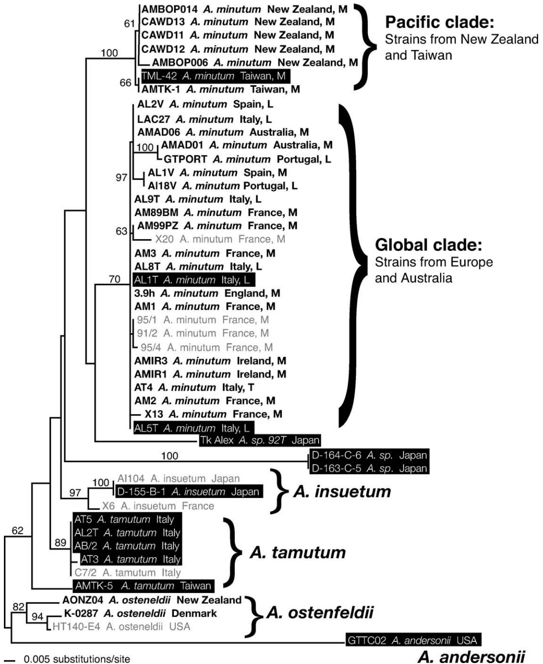
Fig. 6. One of three most likely trees returned by maximum likelihood analysis, score -\ln 2234.15708 . The letter L after a taxon indicates an original morphospecies designation of A. lusitanicum . Bootstrap values are shown behind relevant nodes. Toxic strains are indicated in bold type, non-toxic strains in white type on black. Gray type is used where toxicity is unknown.
