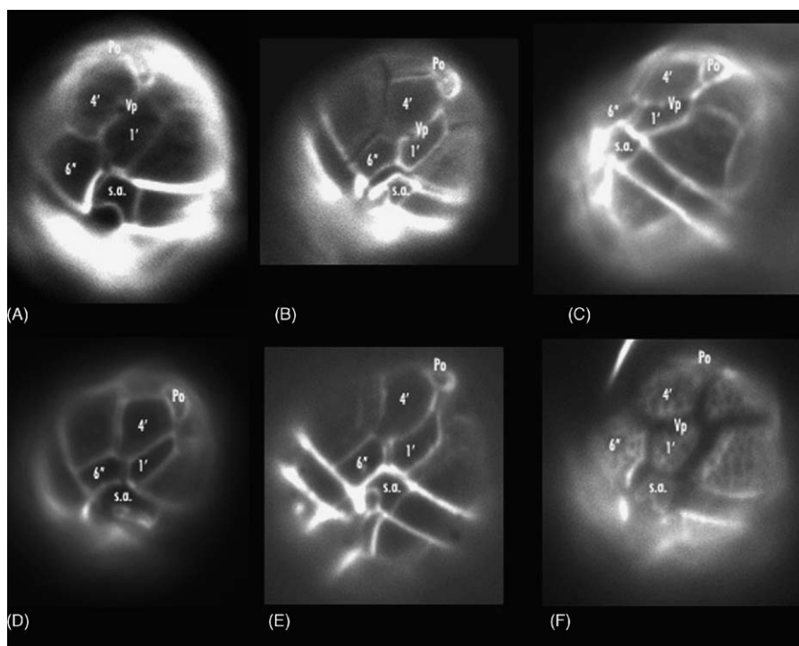
Fig. 4. Examples of the range in connection observed between the Po and 1' plate. (A) Direct connection, A. tamutum AL2T, (B) filamentous connection, A. minutum AL9T, (C) filamentous connection, A. minutum AM3, (D) filamentous connection, A. minutum AM1, (E) direct connection, A. minutum 3.9 h, (F) no connection, A. insuetum D-155-B-1.
