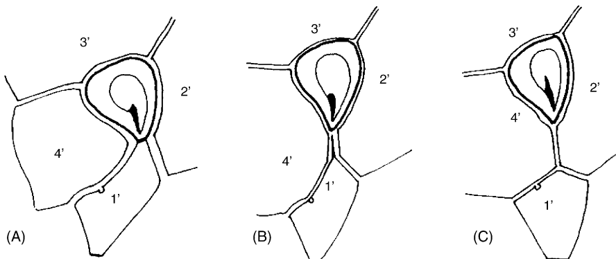
Fig. 2. Differing degrees of connection between the Po and the 1' plate, from Balech (1995). (A) direct connection, (B) filamentous connection, and (C) complete disconnection.
