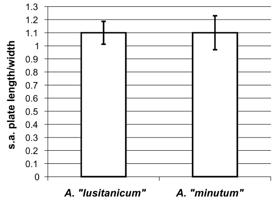
Fig. 3. Average length:width ratios of the anterior sulcal plates for strains designated either A. lusitanicum or A. minutum , Table 2. Error bars are standard deviations.
