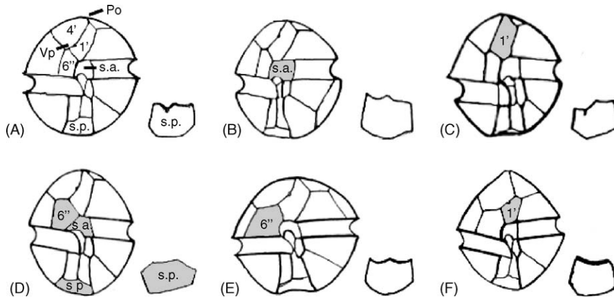
Fig. 1. Plate diagrams showing ventral view and S.p. for the morphospecies discussed in the text, modified from Balech (1995) and Montesor et al. (2004). (A) A. minutum , (B) A. lusitanicum , (C) A. angustitabulatum , (D) A. andersonii , (E) A. tamutum , and (F) A. insuetum . Plate numbers in (A) are after notation described in Balech (1995). In (B–F), gray highlighting indicates key plates that differ from A. minutum .
