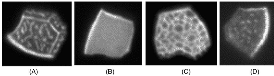
Fig. 5. Examples of the range of thecal plate ornamentation observed. (A) Moderate reticulation, A. sp. D-163-C-5 hypotheca, (B) smooth, unornamented plate, A. sp. D-163-C-5 epitheca, (C) strong reticulation, A. insuetum D-155-B-1, and (D) areolation, A. minutum AM1.
