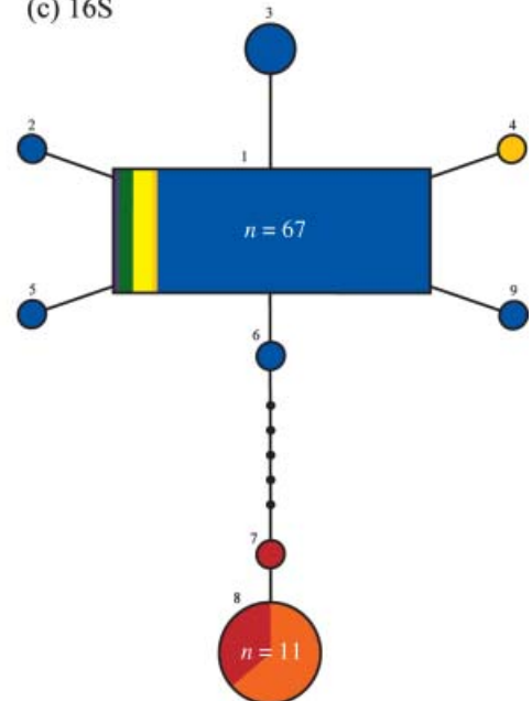
Fig. 3 rcs networks of South American, sub-Antarctic, and Antarctic Parborlasia spp. using the 95% connectivity level. (a) Networks based on concatenated 16S and COI mtDNA genes. (b) Networks based solely on COI mtDNA. (c) Network based solely on 16S mtDNA. Alphanumeric names (designated by letters corresponding to COI sequence and numbers corresponding to 16S sequence) are provided for each haplotype. Sampled haplotypes are indicated by coloured circles or rectangles; missing or unsampled haplotypes are indicated by black dots. Rectangles depict the haplotype with the highest ancestral probability. Each branch indicates a single mutational difference. Circle size is proportional to observed haplotype frequency; observed number of ancestral haplotypes is indicated by 'n = ' (the number of times that haplotype was obtained). Haplotypes are coloured according to the geographical region from which the sample was collected (see legend).
